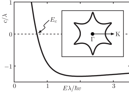
FIG. 2. Curvature c(E) of the equienergy contour in the \Gamma K direction, calculated from Eq. (2.11). The shape changes from convex to concave at energy E_c . The maximally negative curvature is c \approx -1.3\lambda for E \approx 2\hbar v/\lambda , where the equienergy contour has the snowflake-like shape shown in the inset.
